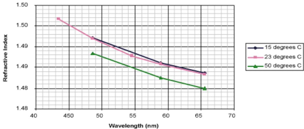
PLEXIGLAS VLD Refractive Index vs. Temperature
